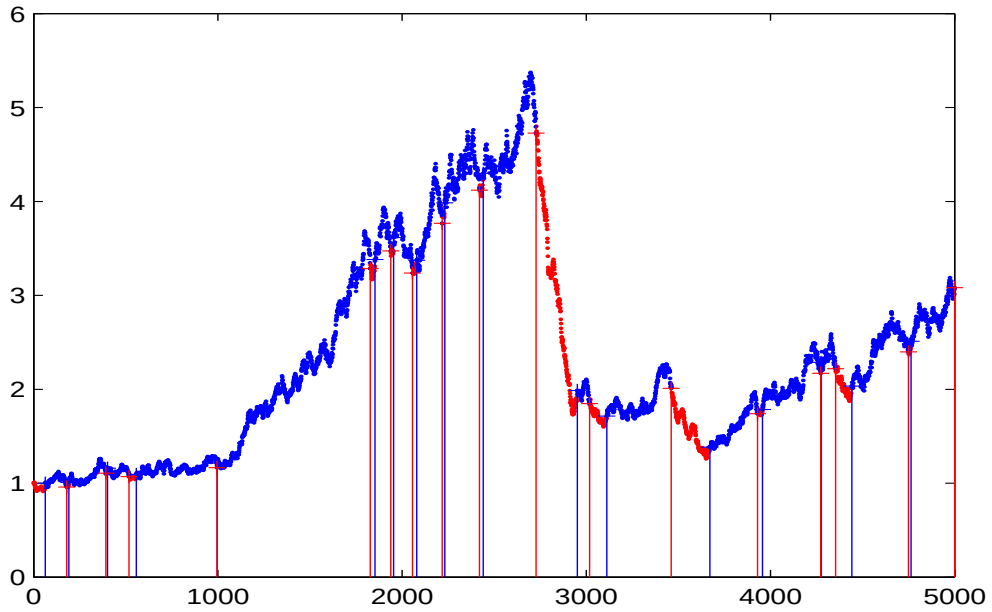
Figure 3: Sample Path
